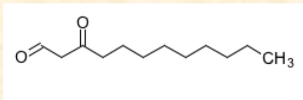
癸醯乙醛
